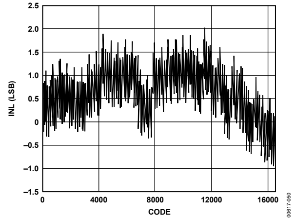
Figure 50. Typical INL
