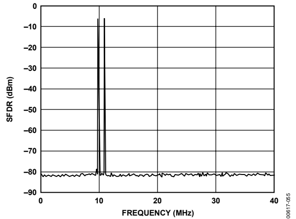
Figure 55. Dual-Tone SFDR @ f_{CLK} = 125 MSPS
