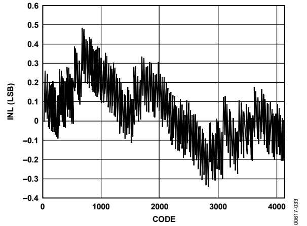
Figure 33. Typical INL
